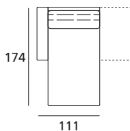
Penisola da 111x174 Dx/Sx Rh/Lh peninsula 111x174
